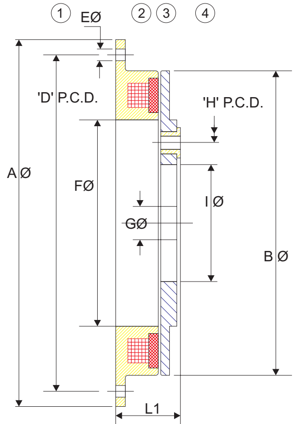
EXTERNAL MOUNTING BRAKE ARMATURE WITHOUT TAPER LOCK
