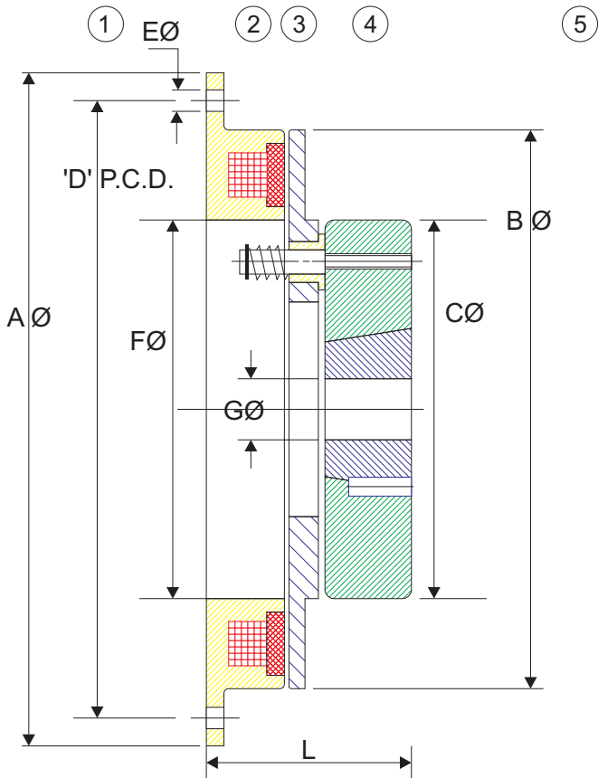
EXTERNAL MOUNTING BRAKE ARMATURE WITH TAPER LOCK
